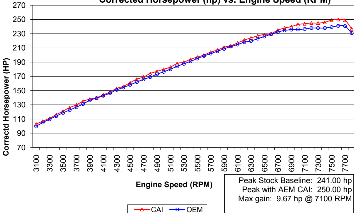
Corrected Horsepower (hp) vs. Engine Speed (RPM)
