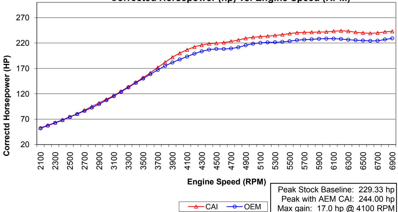
Corrected Horsepower (hp) vs. Engine Speed (RPM)
