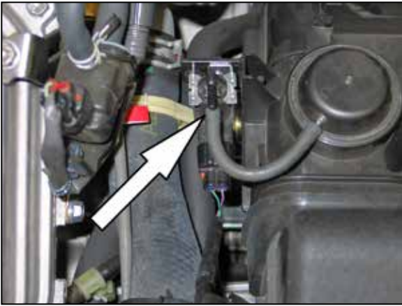
10. Disconnect the lower vacuum hose from the vacuum switching valve.
