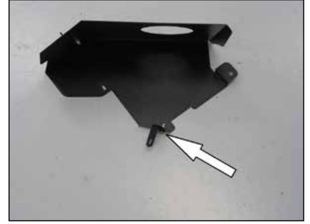
18. Install the heat shield mounting bracket (070812) onto the heat shield using the provided hardware.
