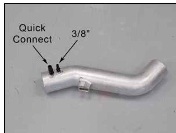
15. Install the Quick connect and 3/8" vent fitting into the K&N® intake tube as shown. NOTE: NPT fittings are easy to cross thread. Install the vent fitting "hand" tight, then turn it two complete turns with a wrench.
