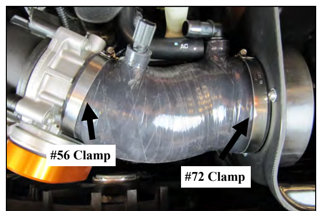
9. Place the #56 and #72 Hose Clamps onto the Airaid Intake Tube and install the assembly leaving the hose clamps loose for now.
