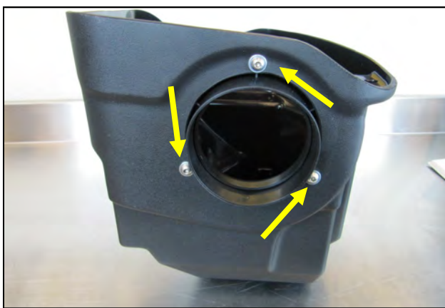
4. Install the Filter Adapter onto the Cool Air Box using the three 1/4" Button Head Screws and 1/4" Flat Washers.
